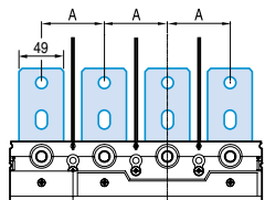
TS800 4P
