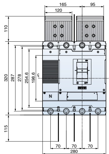
4P (L-type)
